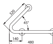
Model lewy - 5181G
