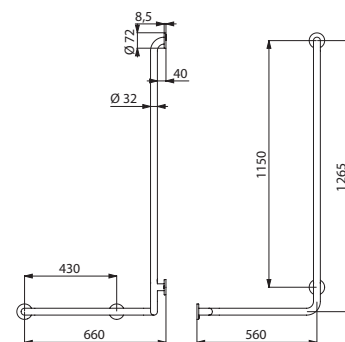
Model lewy - 5100GP2
