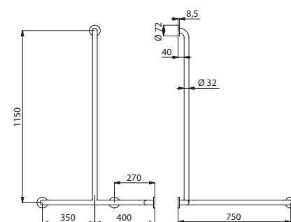
Model lewy - 5481G
